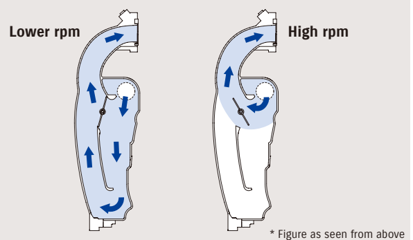
Air Flow in Multi-Stage Induction Module
