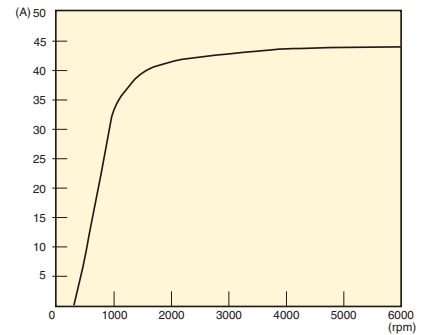
Alternator Output
